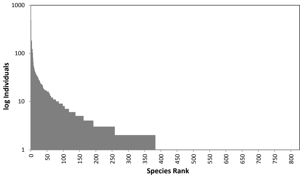
Figure 12. Rank abundance plot for all specimens collected by Malaise trap at Grasslands National Park in 2012.
