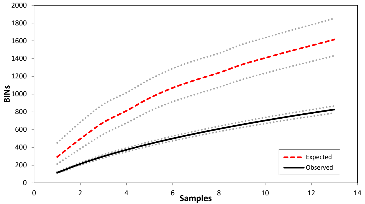
Figure 11. BIN accumulation curve for all specimens collected by Malaise trap at Grasslands National Park in 2012.
