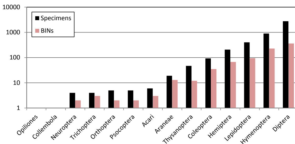
Figure 10. Taxonomic breakdown of specimens collected by Malaise trap at Grasslands National Park in 2012.
